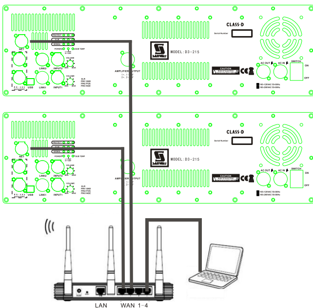
Cable connection
